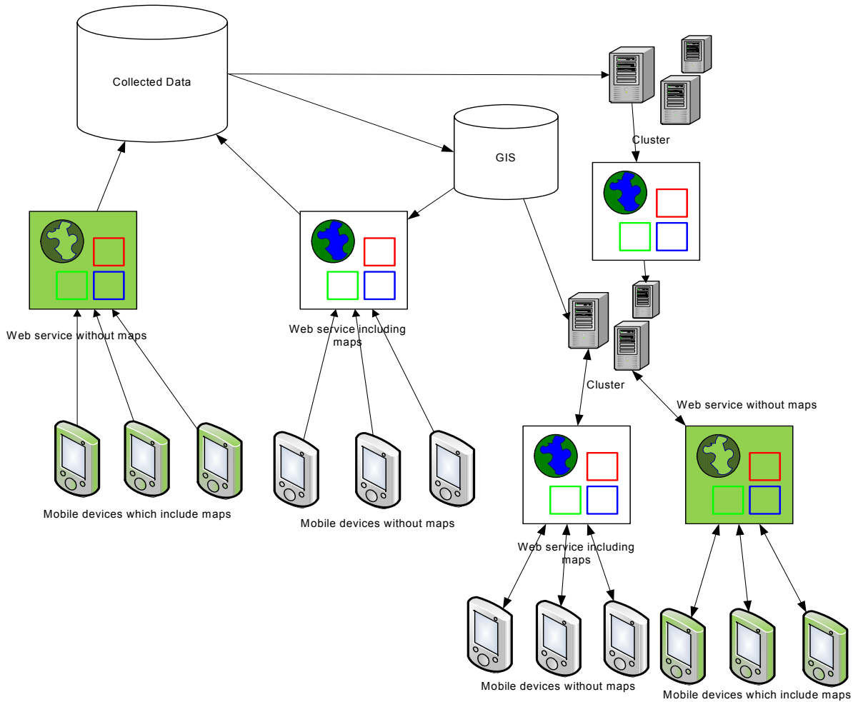
Fig. 1. System architecture
