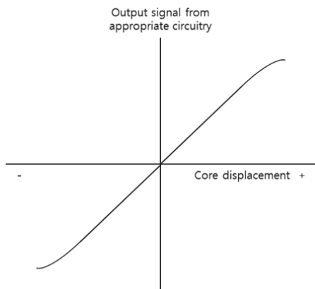
Fig. 4 Output signal from appropriate circuitry
