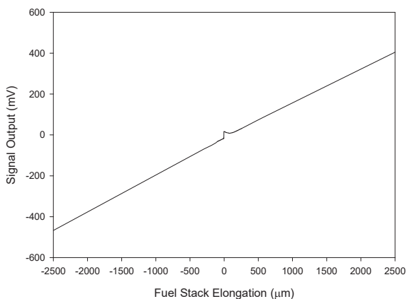
Fig. 8 Signal output from readout
