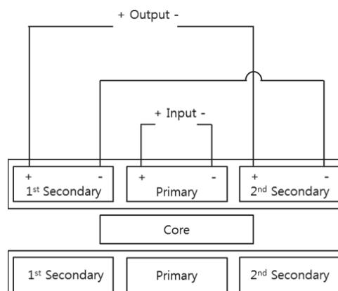
Fig. 1 Cross-sectional view of LVDT core and windings
