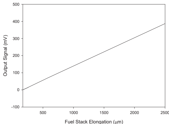
Fig. 10 Feasible measurement range
