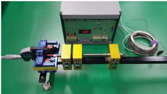
Fig. 7 Experiment for fuel stack elongation measurement
