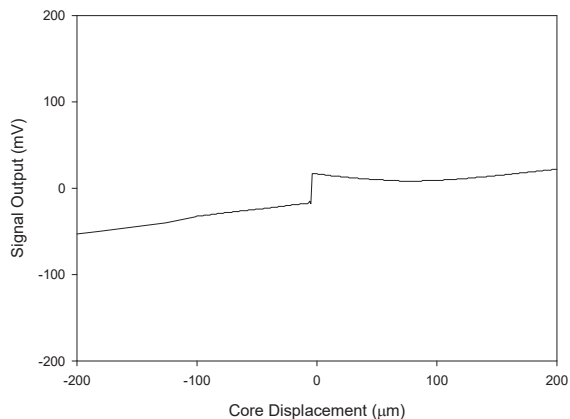
Fig. 9 Nonlinear characteristics at dead zone
