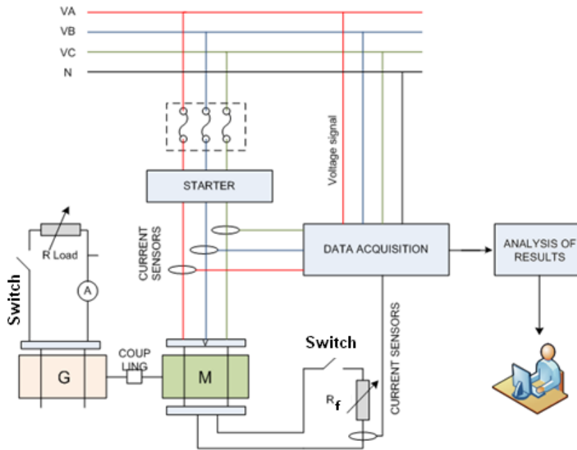
Fig. 6 Laboratory assemblies for fault emulation
