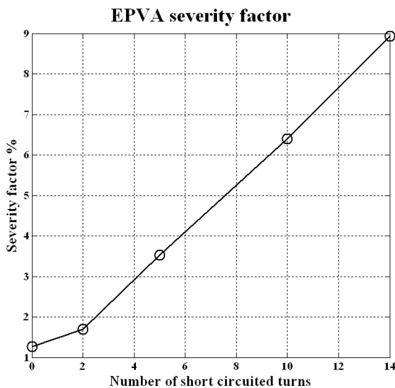
Fig. 18 Severity factor for stator inter-turn short-circuit fault Vs. number of short circuited turns
