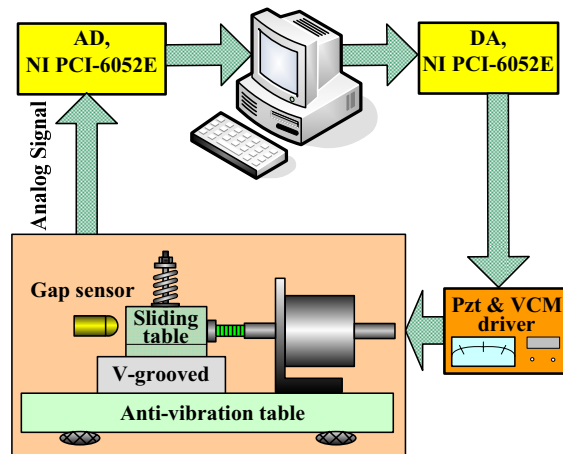
Fig. 9 The schematic drawing of control system.
