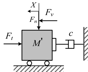
Fig. 2. The mechanical model of the rough positioning.
