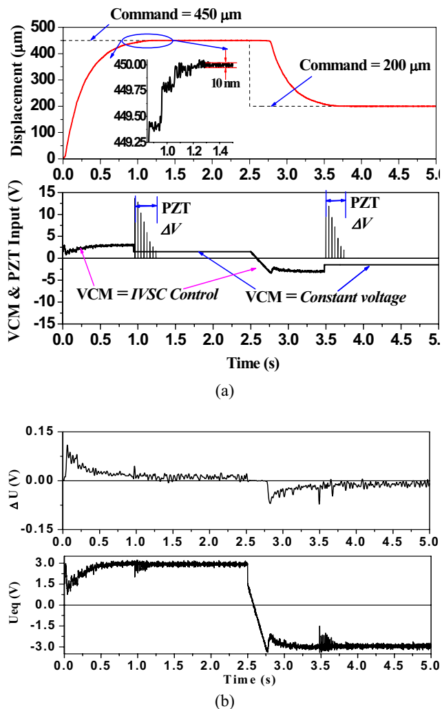
Fig. 10 Experimental results of position control (a) displacement and voltage commands of the piezo-VCM actuators, (b) \Delta U , and equivalent control U_{eq} .
