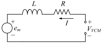
Fig. 3. Theoretical equivalent electrical circuit of the VCM.
