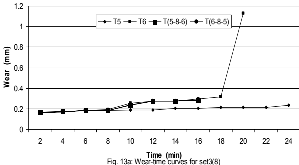
Fig. 13a: Wear-time curves for set3(8)
