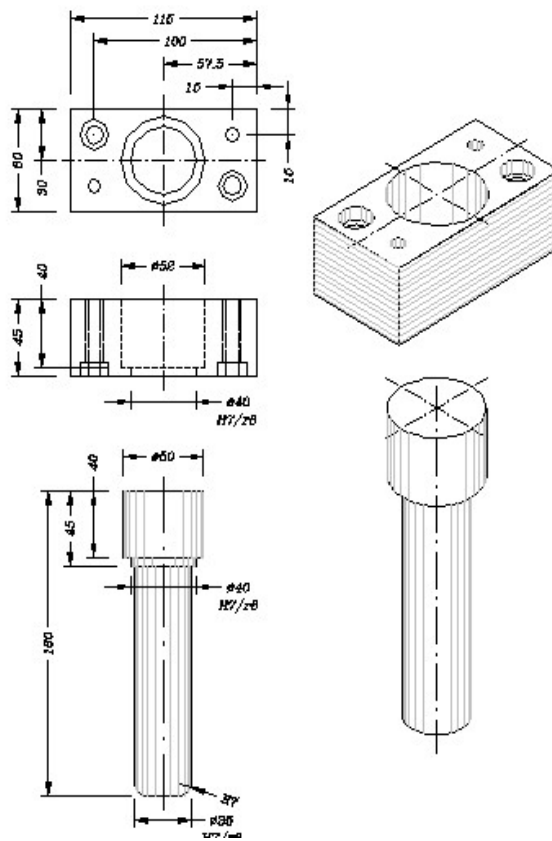
Fig. 6 Guide pillar drawing
