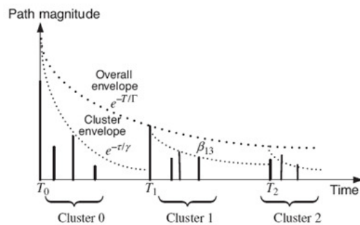
Fig. 4. Saleh-Valenzuela Channel Model
