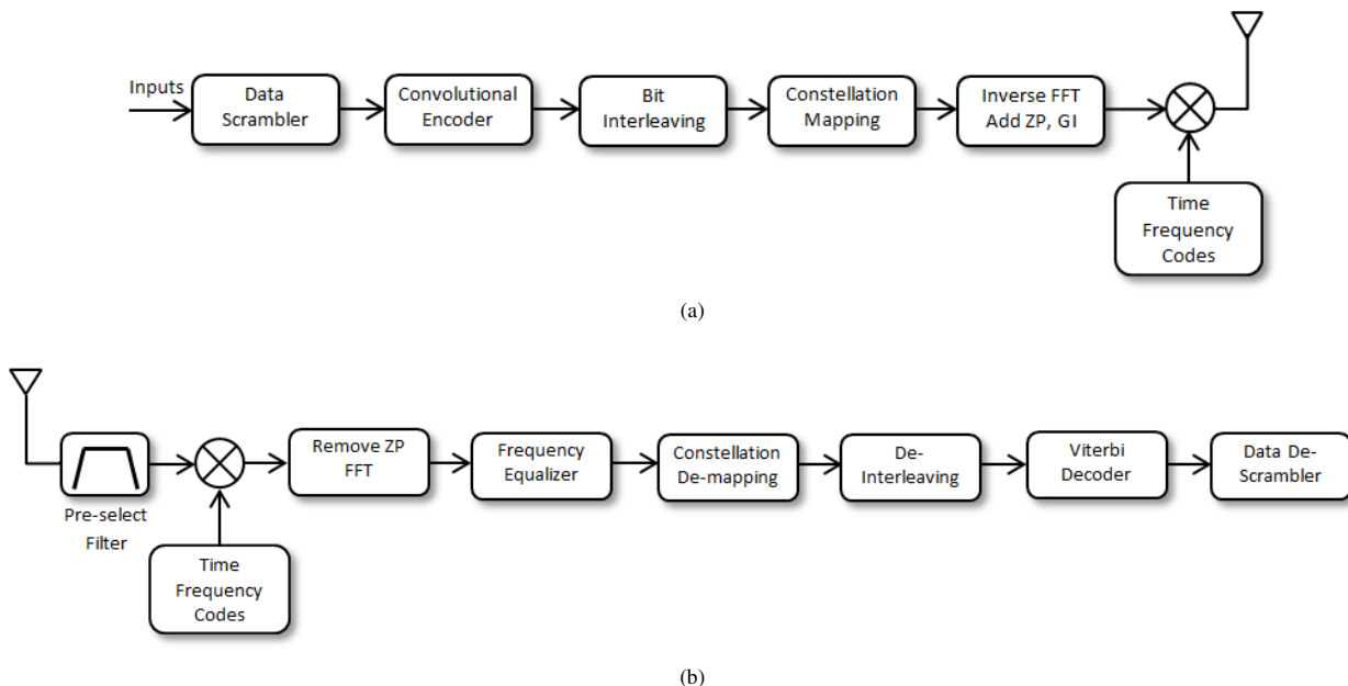
Fig. 5. Multiband OFDM UWB System (a) Transmitter (b) Receiver
