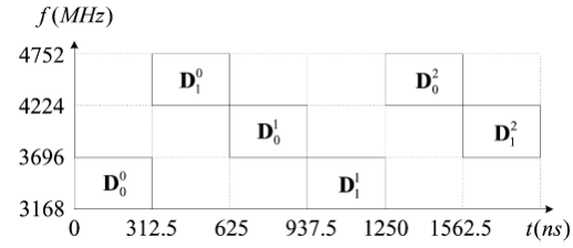
Fig. 3. Time-frequency Coding for Multiband OFDM System
