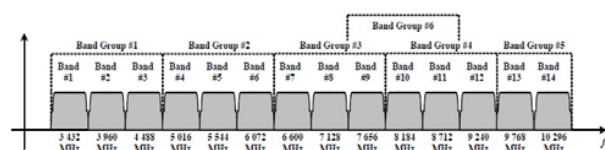
Fig 1. UWB Frequency Band Planning
