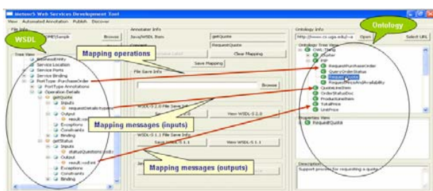
Fig. 4 Annotating Web services with ontological concepts
