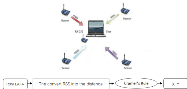
Fig. 2 Structure of the indoor positioning system
