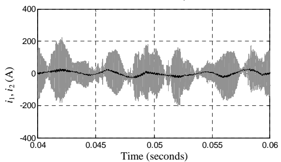
Fig. 11 Input (in gray) and output (in black) currents of the LCL filter for L_2= 4mH , C_f=0.6\mu F and L_1=0.1mH
