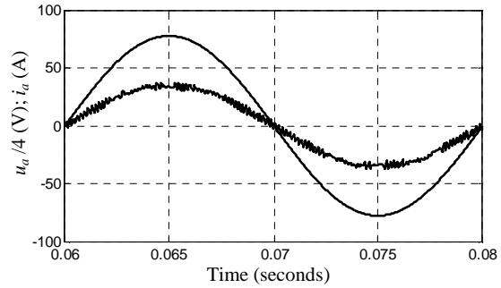
Fig. 9 Waveforms of supply voltage and current for L_2= 4mH and C_f=0.6\mu F
