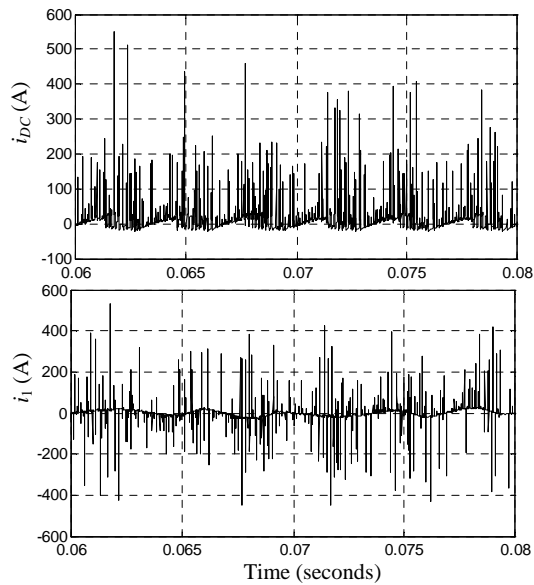
Fig. 10 DC-side current and VSC output current for L_2= 4mH and C_f=0.6\mu F
