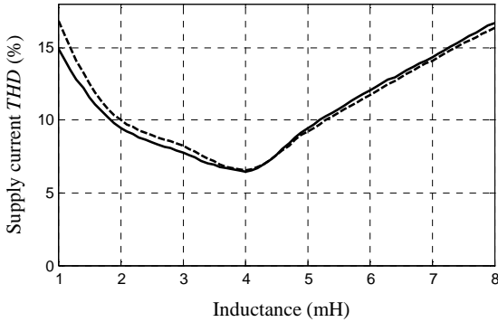
Fig. 7 Supply current THD versus inductance L_2 for C_f=0.6\mu F (solid line) and C_f= 3\mu F (dashed line)
