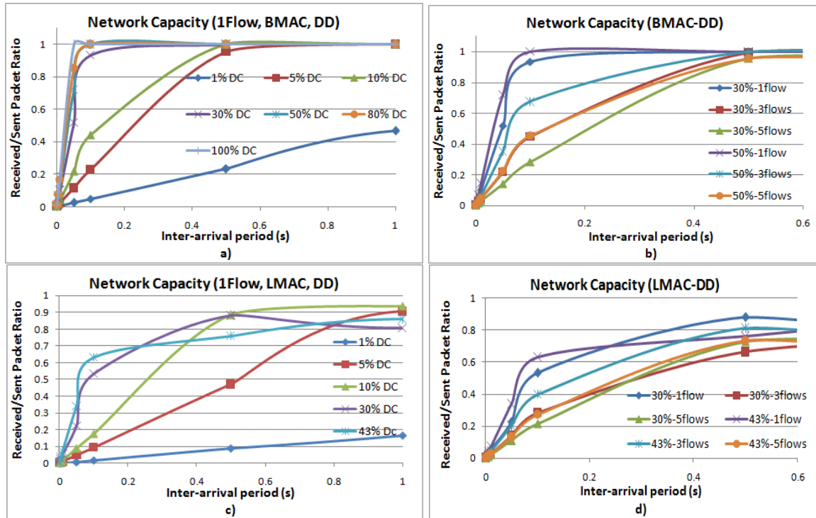
Figure 2: Successful Transmission Measurements Excluding Routing Protocol Overhead
