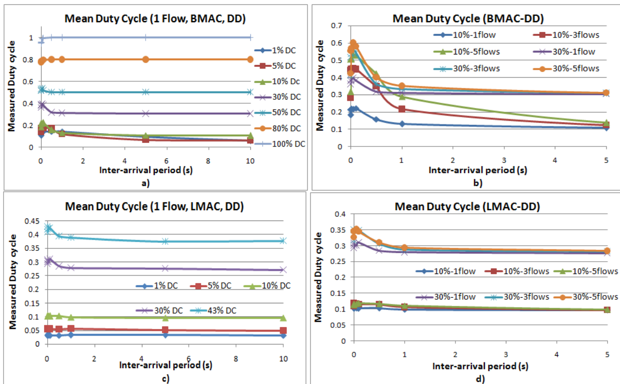
Fig. 4 Effective Duty Cycle Measurements Excluding Routing Protocol Overhead
