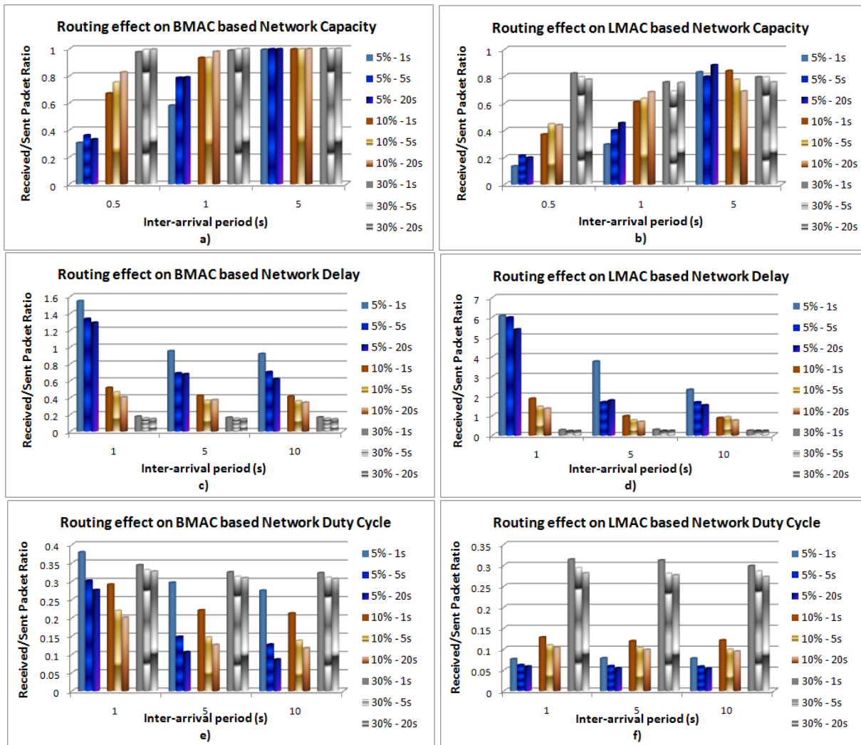
Fig. 5 The Routing Overhead Effect on Delay and Effective DC Performance
