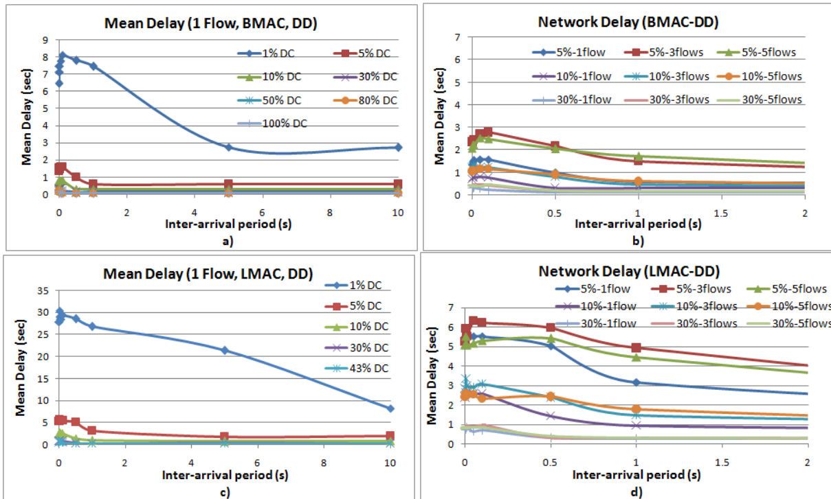
Fig. 3 Mean Packet Delay Measurements Excluding Routing Protocol Overhead
