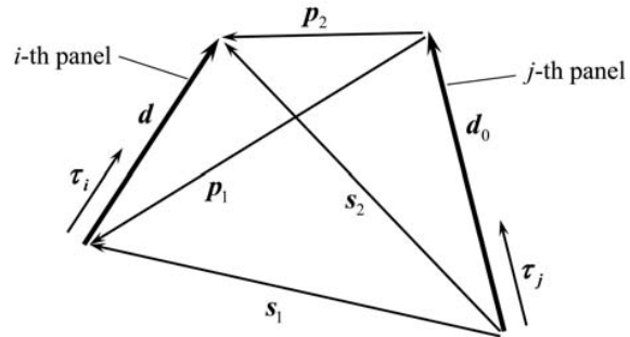
Fig. 1. Two panels from airfoil surface and auxiliary vectors
