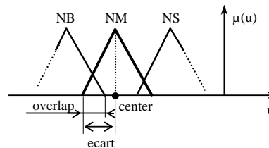
Fig. 3 Description of membership function parameters
