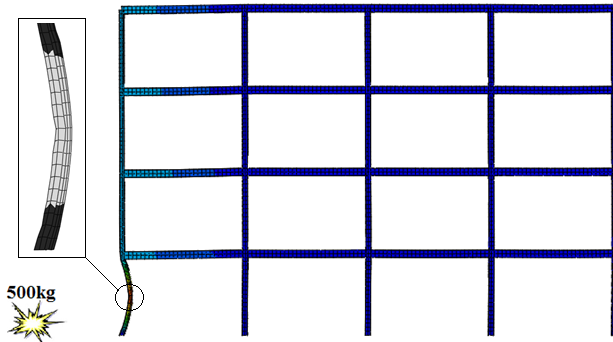
Fig. 20 Typical in-plane frame's response
