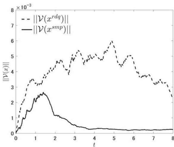
Fig. 6 Time responses of \|\mathcal{V}(x^{rdq})\| and \|\mathcal{V}(x^{smp})\| .
