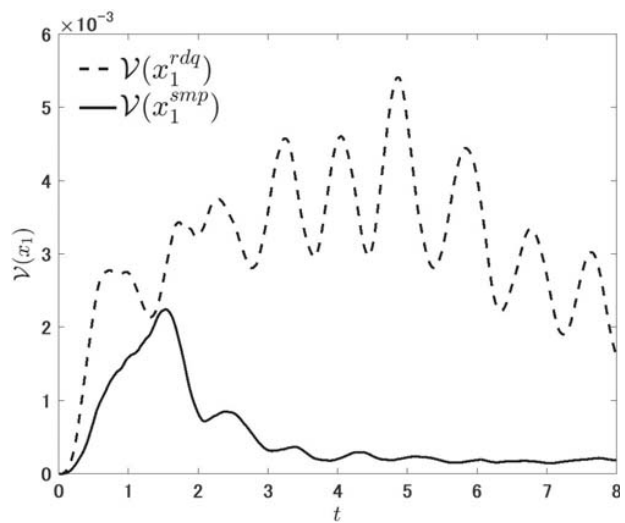
Fig. 3 Time responses of \mathcal{V}(x_1^{rdq}) and \mathcal{V}(x_1^{smp}) .
