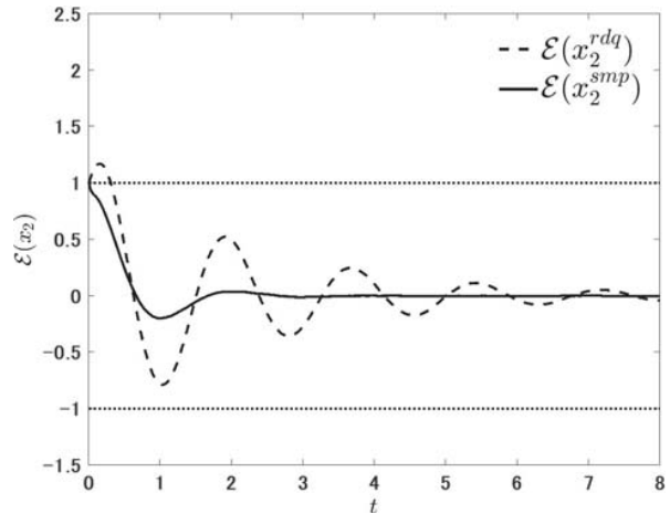
Fig. 2 Time responses of \mathcal{E}(x_2^{rdq}) and \mathcal{E}(x_2^{smp}) .
