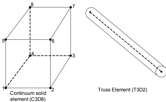
Fig. 1 Elements used in model development [17]
