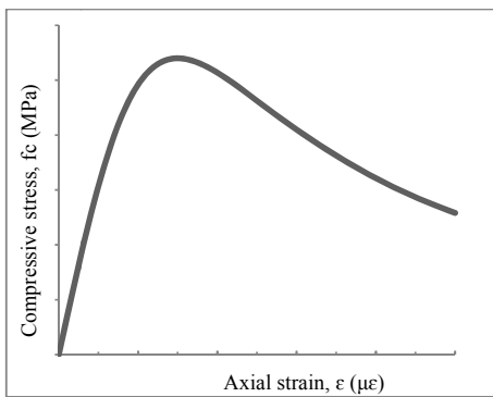
Fig. 5 Uniaxial Compressive Stresses for 27 MPa Concrete
