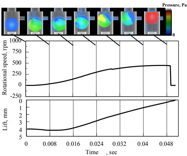
Fig.7 Relationship between the rotational speed and lift of the Center model (12 cm 3 /s)
