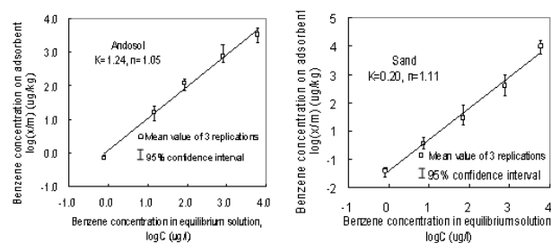
Fig. 2 Freundlich plot for benzene on Andosol (upper figure) and sand (lower figure).
