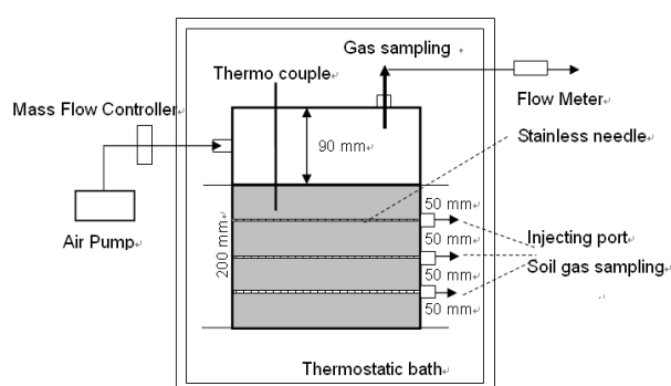
Fig.1 Schematic diagram of the flux chamber
