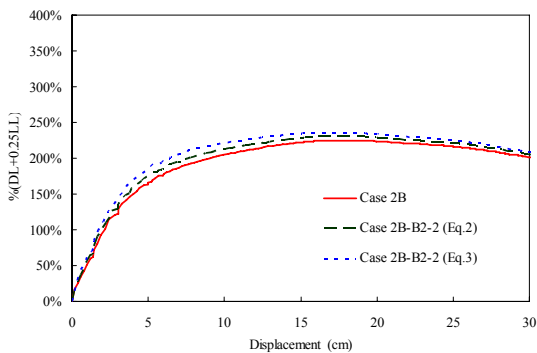
Fig. 8(c) Pseudo-static response curves of Case 2B-B2-2
