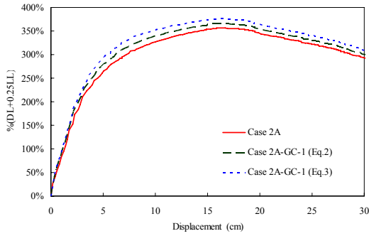
Fig. 7(b) Pseudo-static response curves of Case 2A-GC-1
