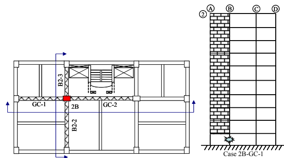
Fig. 2(c) Locations of brick infill in Case 2B
