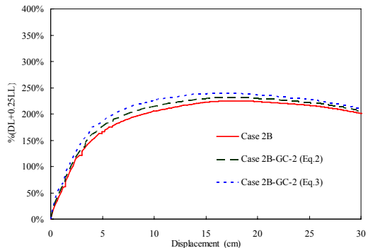
Fig. 8(b) Pseudo-static response curves of Case 2B-GC-2
