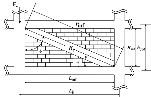
Fig. 3 Loading direction of the brick infill
