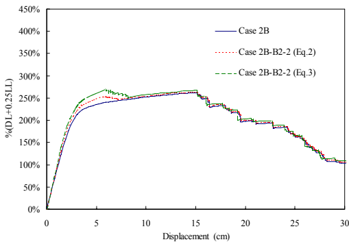
Fig. 6(c) The load-displacement responses of Case 2B-B2-2
