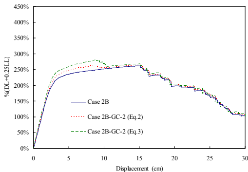
Fig. 6(b) The load-displacement responses of Case 2B-GC-2
