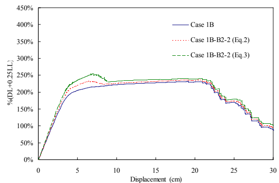
Fig. 5(a) The load-displacement responses of Case 1B-B2-2
