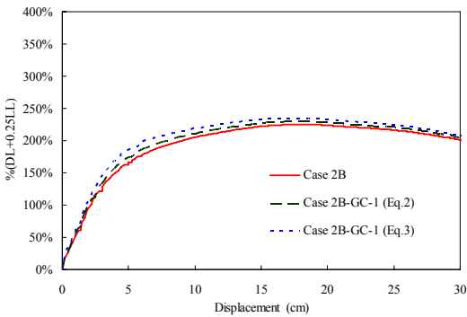
Fig. 8(a) Pseudo-static response curves of Case 2B-GC-1
