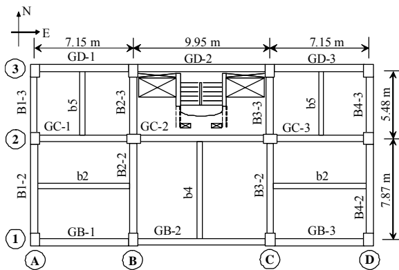
Fig. 1 Plan dimensions of the building
