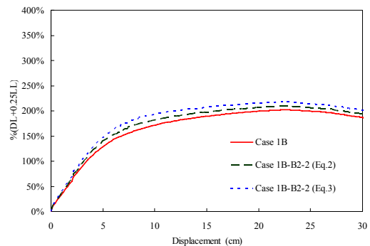
Fig. 7(a) Pseudo-static response curves of Case 1B-B2-2
