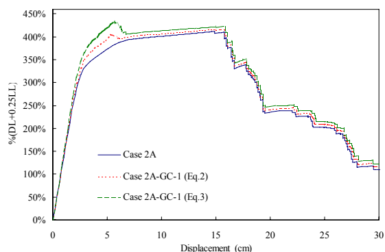
Fig. 5(b) The load-displacement responses of Case 2A-GC-1
