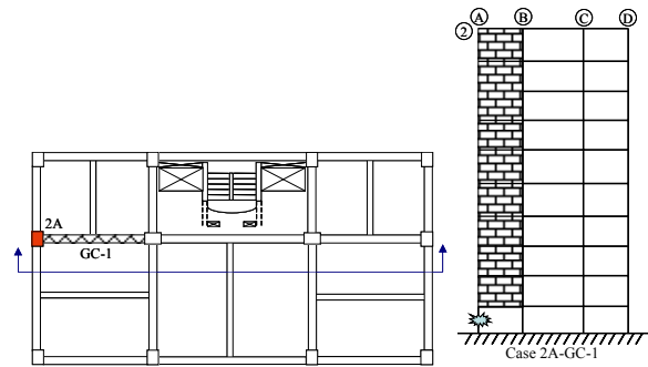
Fig. 2(b) Location of brick infill in Case 2A
