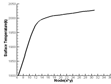
Fig. 3 Temperature variation of the surface central point versus number of the nodes
