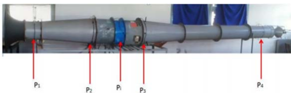
Fig. 2 Test bench realized, p: static pressure
