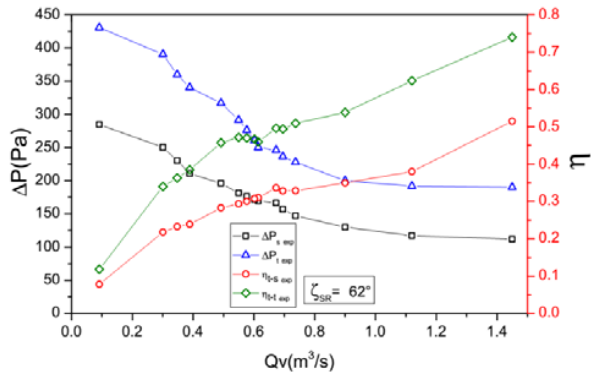
Fig. 9 Pressure elevation and efficiency ( \xi_{SR} = 62^\circ )
