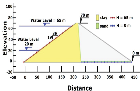
Fig. 3 Dam's geometry
