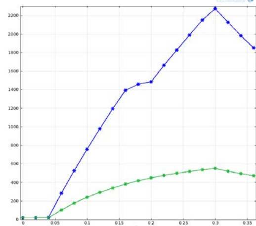
Fig. 11 Temperature changing history at two locations for Case: 3 current 19.2kAmps
