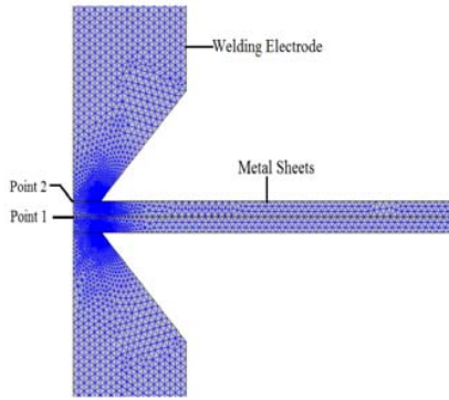
Fig. 2 Geometry meshing
