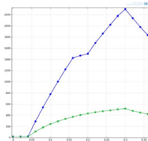
Fig. 4 Temperature changing history at point 1 and point 2 for case :1 12kAmps
