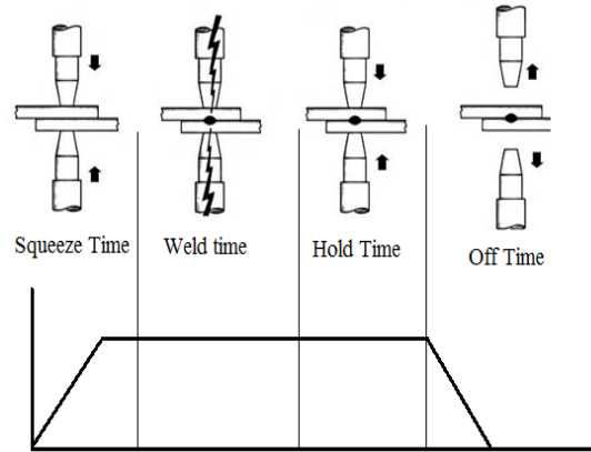
Fig. 1 Complete spot weld cycle
