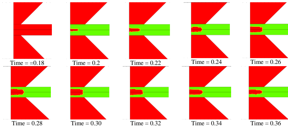
Fig. 12 Welding nugget formation for Case: 3 (19.2kAmps) with tip contact area of 201.06 mm 2
