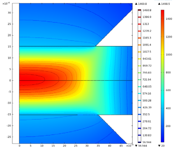
Fig. 3 Thermal profile at faying surface
