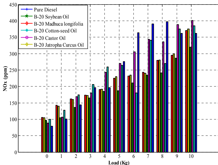
Fig. 1 Variation of NO x emissions with respect to engine loading
