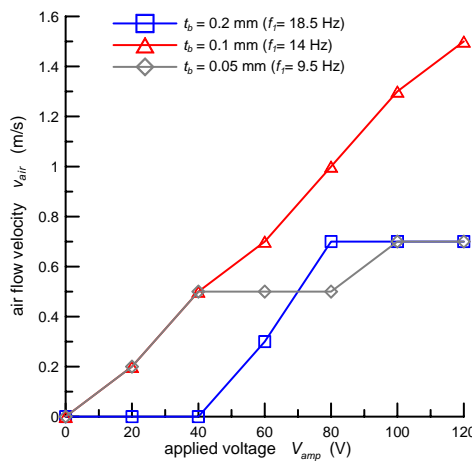
Fig. 11 Relationship between v_{air} and V_{amp} of piezoelectric fan with steel blade
