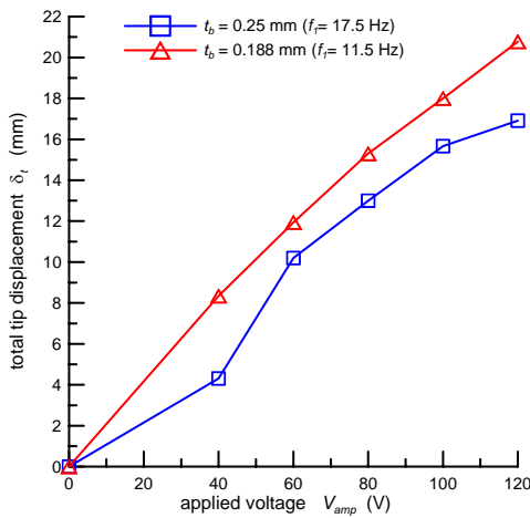
Fig. 10 Relationship between \delta_t and V_{amp} of piezoelectric fan with PET blade
