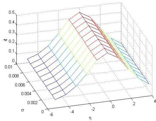
Fig. 3 Solitary profiles for different value of \sigma
