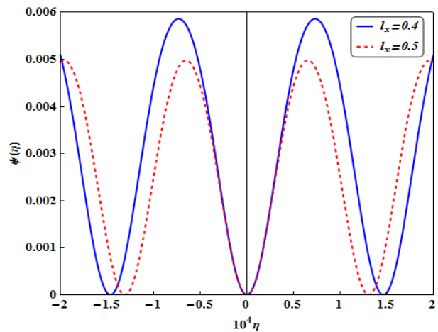
Fig. 6 Variation of periodic travelling wave \Psi versus \eta for \chi = 2 , \delta = 0.2 , \gamma_{xce,p} = 0.4 , \lambda_{xce,p} = 0.1 , U = 0.4 and \Omega_c = 0.004
