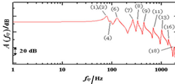
Fig. 13 Fourier spectrum of impact response for “High Stiffness Elastic Frame Model with Damping Layer” under small input ( |f_{\max}|=0.98(\text{N}) )
