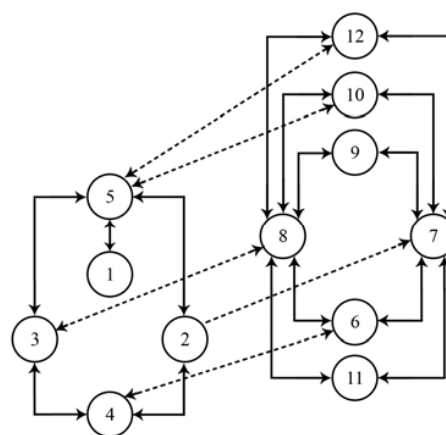
Fig. 4 The flow pattern of the configuration probability. The notations are the same as in Fig. 2-3. The dash-line represents the interchange of the probabilities between two circles. The probability flow can be determined by the effect of the direction of the external field, i.e. for our system with external field, the direction of
