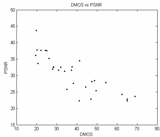
Fig. 5 PSNR compared with DMOS using training images
