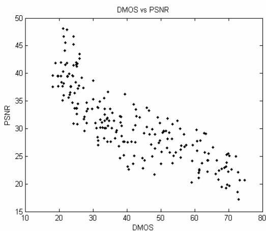
Fig. 7 PSNR compared with DMOS using testing images
