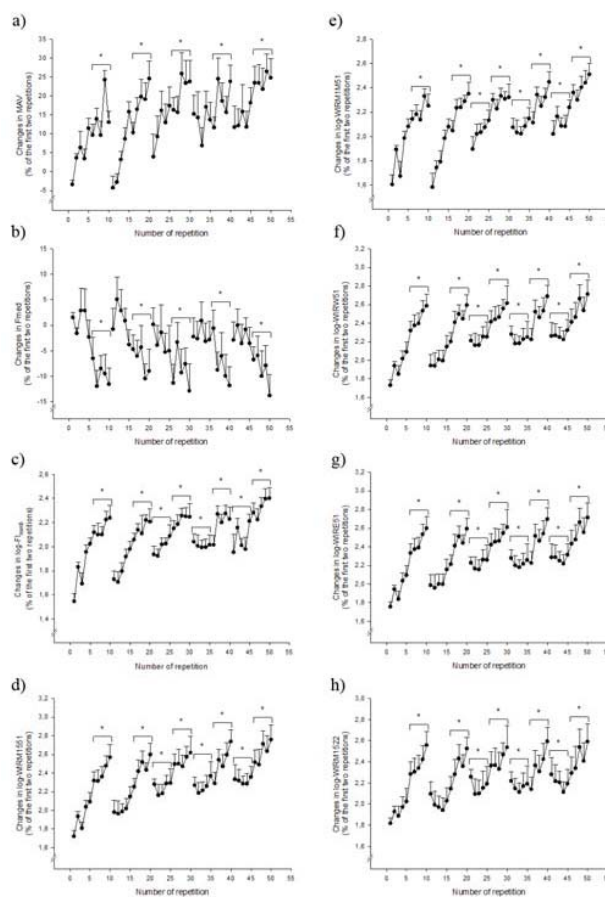
Fig.3. Changes in sEMG parameters (mean \pm standard error) during the 5 sets of 10 repetitions. a) Average MAV b) Median frequency c) Logarithm of Dimitrov's index ( FI_{nsm5} ) d) Logarithm of WIRM1551 e) Logarithm of WIRM1551 f) Logarithm of WIRW51 g) Logarithm of WIRE51 h) Logarithm of WIRM1522.
