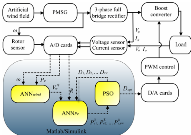
Fig. 6. Block diagram of the MPPT control System.
