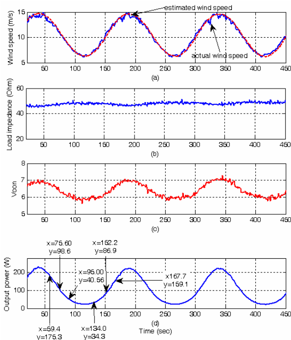
Fig. 11. MPPT result under sinusoidal wind speed and fixed load impedance. (a) Wind speed. (b) Load impedance. (c) V con . (d) Output power.
