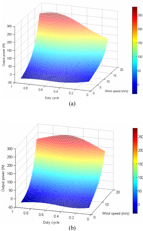
Fig. 9. Three-dimensional curve of ANN_{Pe} . (a) Load impedance 50 \Omega . (b) Load impedance 30 \Omega .
