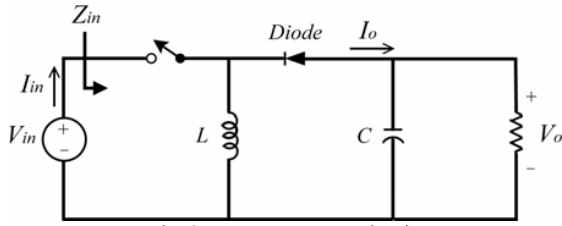
Fig. 3. Boost converter circuit.
