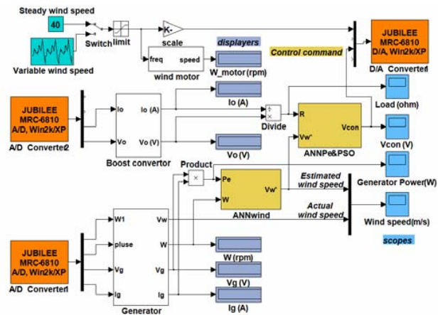
Fig. 7. Simulink structure of MPPT control.
