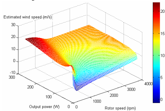
Fig. 8. Three-dimensional curve of ANN wind .
