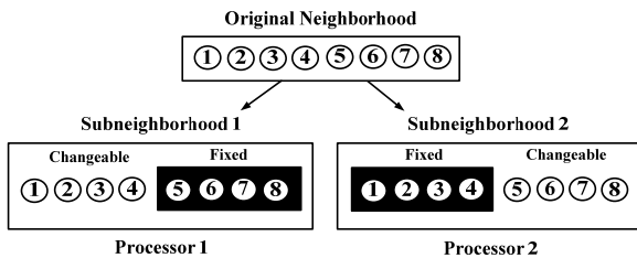
Fig. 3 Search direction of Tabu search
