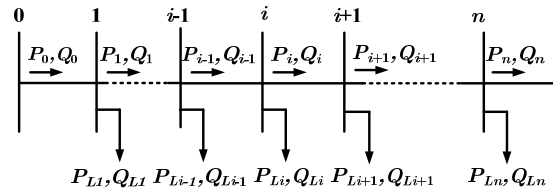
Fig. 1 Single-diagram of main feeder
