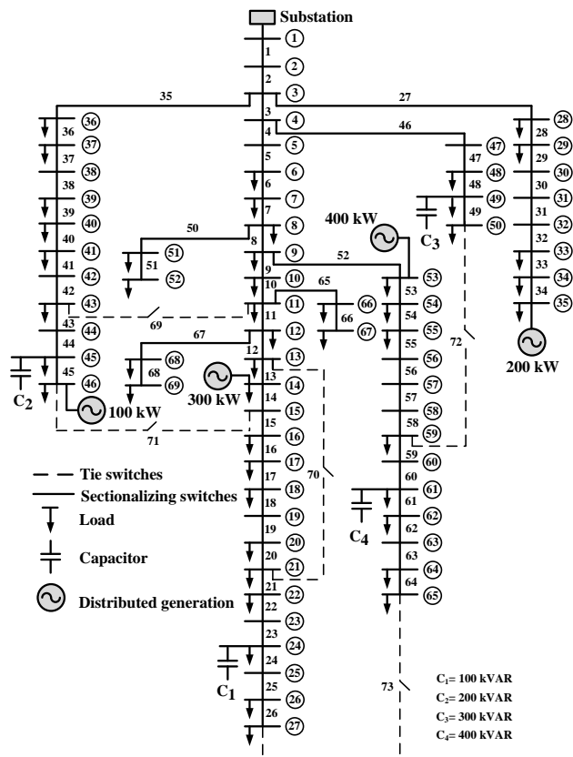
Fig. 5 Test system of 69-bus radial distribution with distributed generation and capacitor placements
