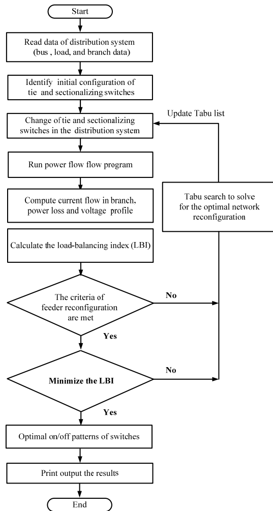
Fig. 4 Flowchart of network reconfiguration for load balancing
