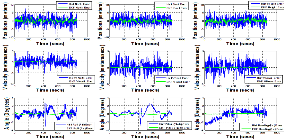
Fig. 1 H^\infty/KF performance in presence of known errors
