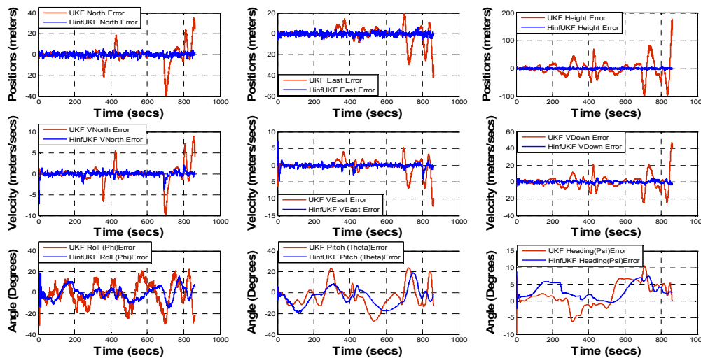
Fig. 5 H^\infty UKF/UKF performance in presence of colored noise
