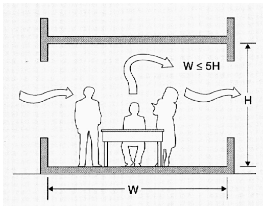
Fig 2 Cross-ventilation [27]
