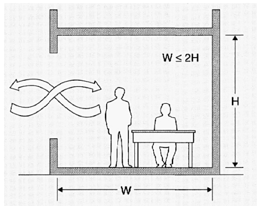
Fig. 1 Single-sided ventilation [27]
