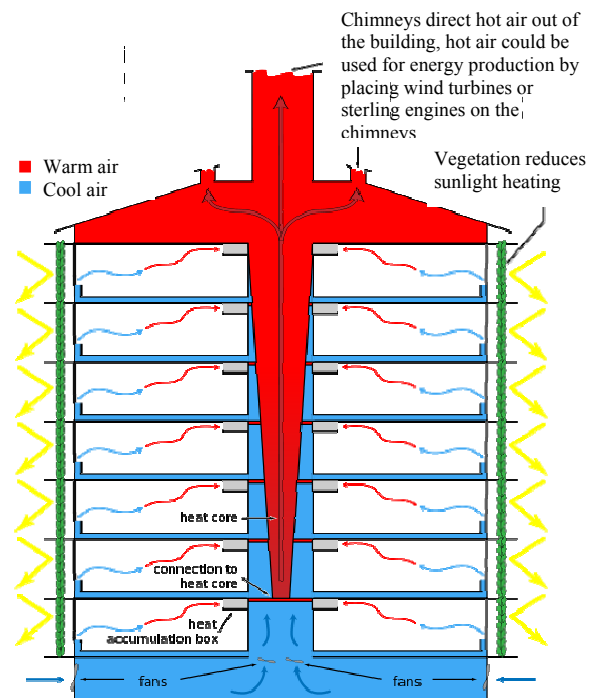
Fig 3 Stack effect for natural ventilation in tall buildings [20]
