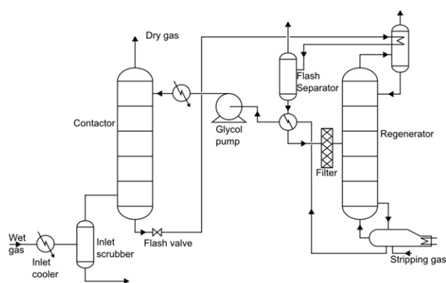
Fig. 1 Typical gas dehydration process
