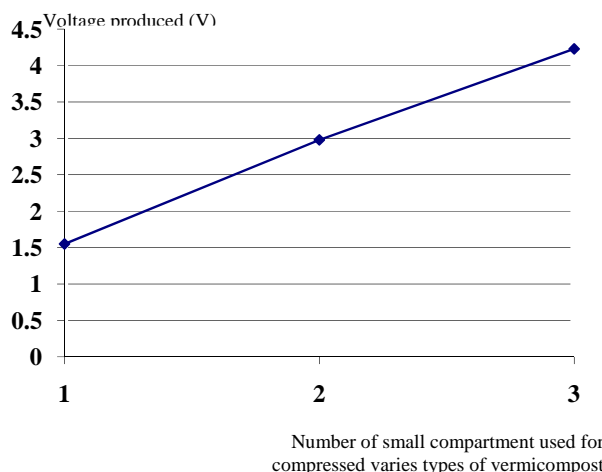
Fig. 4 Relationship between compressed vermicompost and the voltage produced
