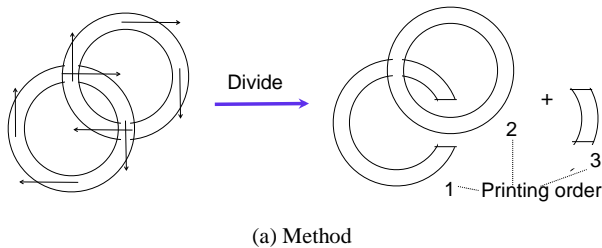
(a) Method
