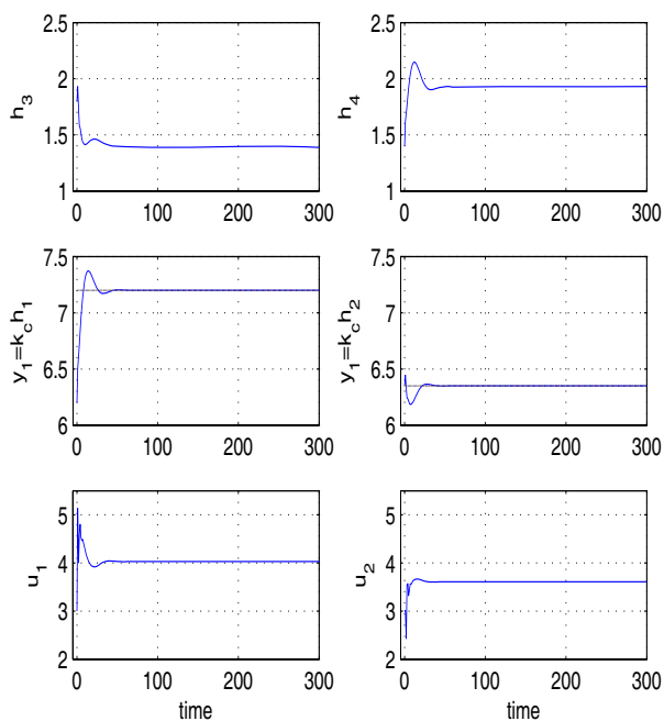
Fig. 3. Predictive PID design for minimum phase
