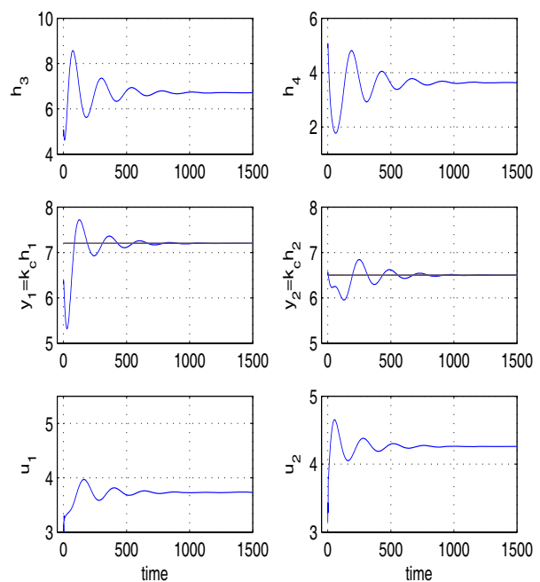
Fig. 5. Predictive PID design for non-minimum phase
