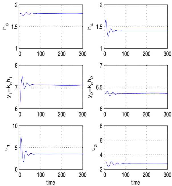
Fig. 2. Manual PID design for minimum phase
