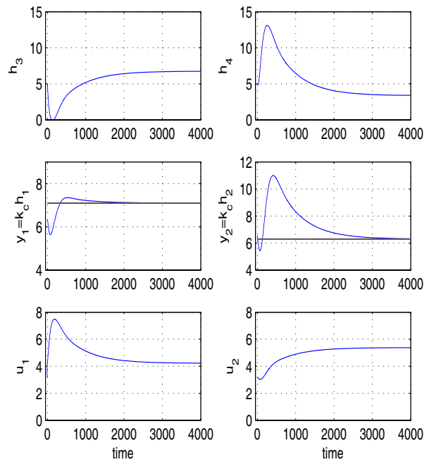
Fig. 4. Manual PID design for non-minimum phase
