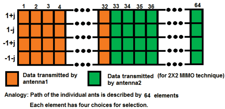
Fig. 4 Illustration of Pheromone matrix used in proposed scheme
