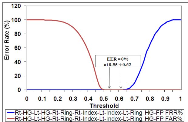
Fig. 25 Extracted EER for our Rt-Lt-HG-FP MMBS
