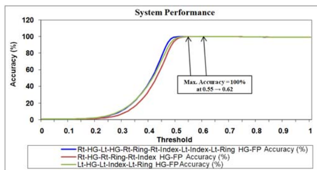
Fig. 26 Comparison between the accuracy for Rt-HG-FP, Lt-HG-FP, and Rt-Lt-HG-FP MMBSs
