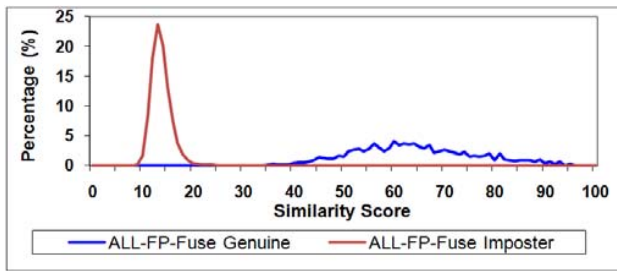
Fig. 16 Identification test for genuine and imposter similarity score distributions of multi-instance Rt-Lt-FP biometric system using our minutiae feature fusion scheme
