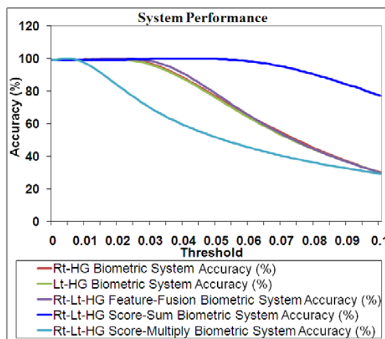
Fig. 8 Accuracy for our HG single-modality and bi-instance biometric systems
