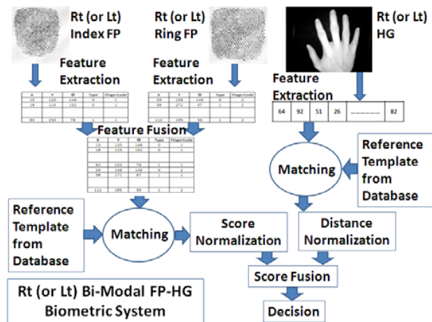
Fig. 17 Schematic for Rt-HG-FP (or Lt-HG-FP) MMBS
