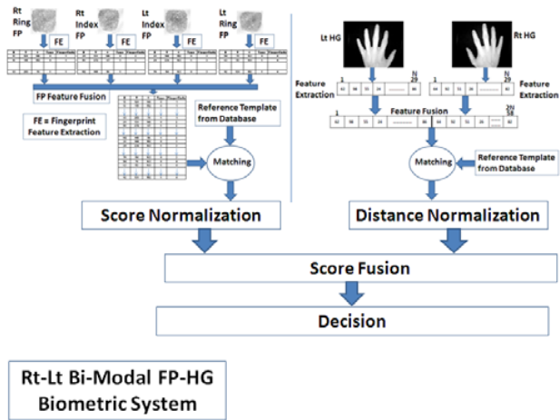
Fig. 24 Schematic for Rt-Lt-HG-FP MMBS
