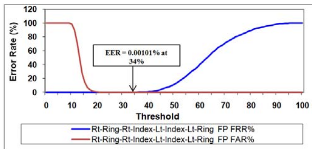
Fig. 13 FAR versus FRR and extracted EER for Rt- Lt (using our minutiae feature fusion scheme) multi-instance FP system
