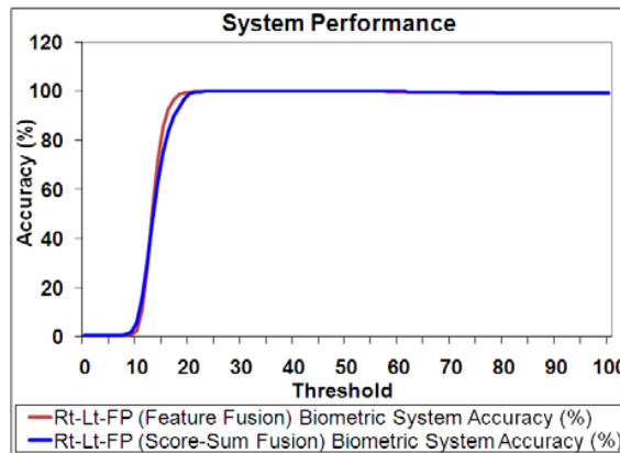
Fig. 14 Accuracy for our Rt-Lt multi-instance FP systems
