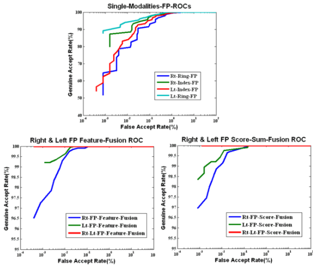
Fig. 15 ROC curves for the 4 single-modality (up), ROC curves for the 3 bi- and multi-instance (using our FP feature-level fusion method) (bottom left), and ROC curves for the 3 bi- and multi-instance (using sum-of-scores score-level fusion technique) FP biometric systems (bottom right)
