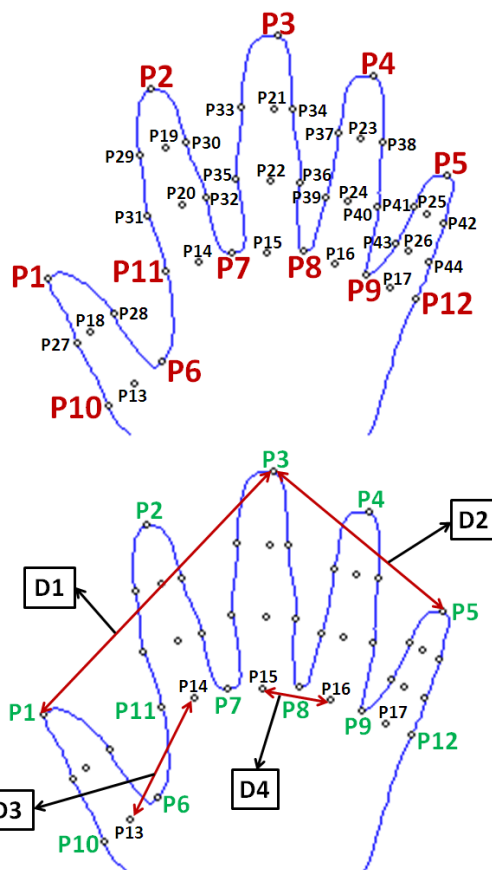
Fig. 5 Automatically detected 44 point hand model (P1-P5 Maximas, P6-P9 Minimas), (Up). Rt/Lt automatic hand type differentiation algorithm: If (D1 > D2) AND/OR (D3 > D4) then image is for Rt HG, otherwise image is for Lt HG, (Bottom)
