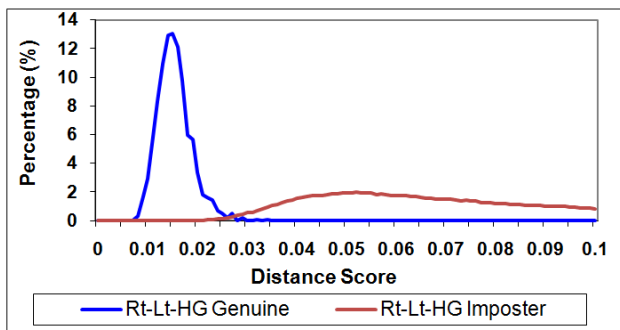
Fig. 10 Genuine and imposter distance score distributions for Rt-Lt-HG (Feature-Level Fusion) bi-instance biometric system
