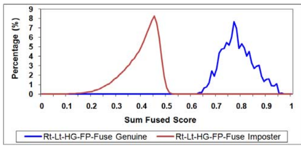
Fig. 28 Identification test for genuine and imposter sum fused score distributions of Rt-Lt-HG-FP MMBS
