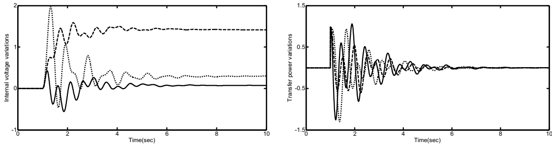
Fig. 9. Internal voltage and transfer power variations of generators; Solid ( G_3 ), Dashed ( G_2 ) and Dotted ( G_1 ).
