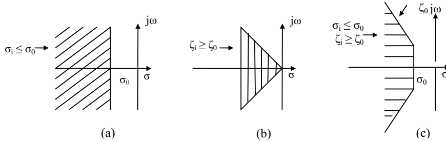
Fig. 1. Region of eigenvalue location for objective function.
