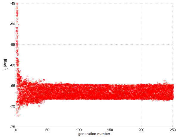
Fig. 25 \beta_{2c} vs. generation number – 2 nd optimization
