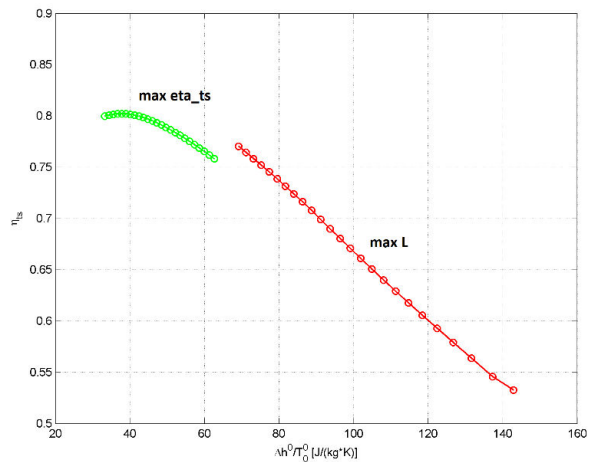
Fig. 5 \eta_{ts} vs. \Delta h^0 / T_0^0 – Maximum \eta_{ts} and maximum L individuals – Pareto front of last generation – 1 st optimization
