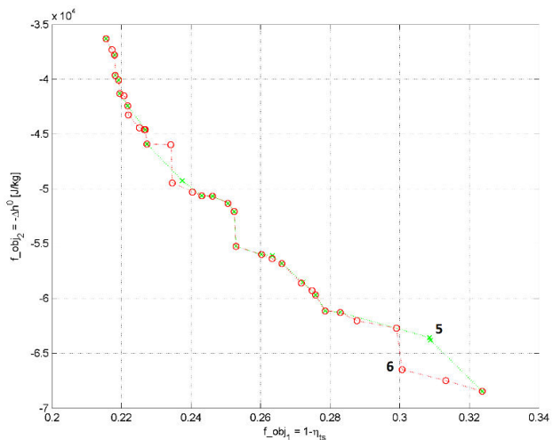
Fig. 3 Pareto front at 5 th and 6 th generations – 1 st optimization
