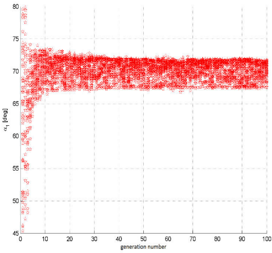
Fig. 6 \alpha_{1c} vs. generation number – 1 st optimization
