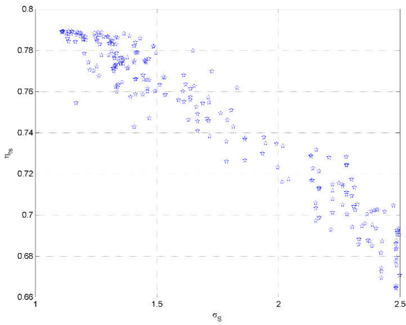
Fig. 28 \eta_{ts} vs. \sigma_s – last Pareto front – 2 nd optimization
