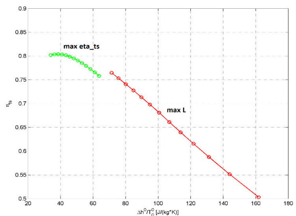
Fig. 21 \eta_{ts} vs. \Delta h^0 / T_0^0 – Maximum \eta_{ts} and maximum L individuals – Pareto front of last generation – 2 nd optimization
