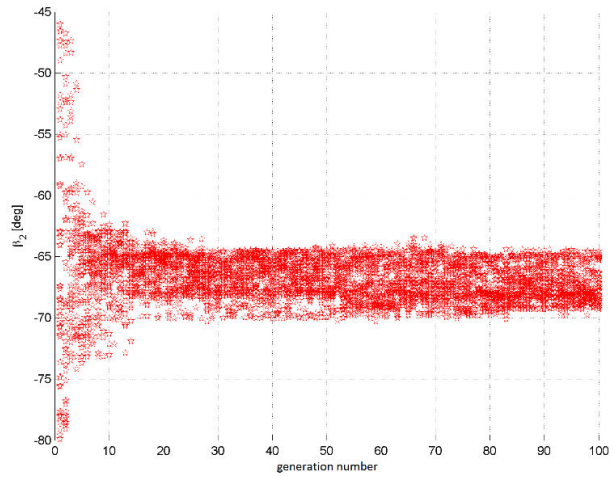
Fig. 9 \beta_{2c} vs. generation number – 1 st optimization
