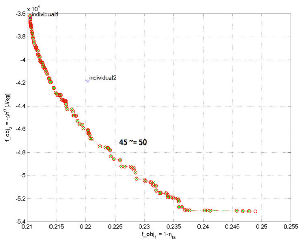
Fig. 39 Pareto front at 45 th and 50 th generations – 1 st local optimization (maximum efficiency)
