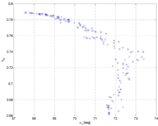
Fig. 11 \eta_{ts} vs. \alpha_{1c} – last Pareto front – 1 st optimization
