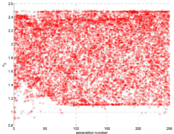
Fig. 26 \sigma_R vs. generation number – 2 nd optimization
