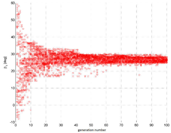
Fig. 8 \beta_{1c} vs. generation number – 1 st optimization
