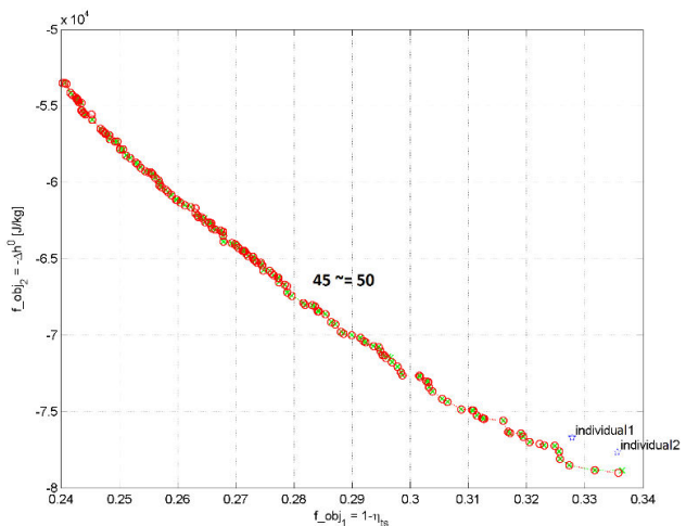
Fig. 41 Pareto front at 45 th and 50 th generations – 3 rd local optimization (maximum specific work)
