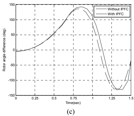
Fig. 8 Variation of generator – 10(11 bus system) rotor angle difference without and with IPFC for different fault clearing times( t_c ), (a) t_c = 0.65 (b) t_c = 0.75 (c) t_c = 0.7
