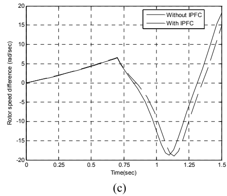
Fig. 9 Variation of generator – 10(11 bus system) rotor speed difference without and with IPFC for different fault clearing times( t_c ), (a) t_c = 0.65 (b) t_c = 0.75 (c) t_c = 0.7
