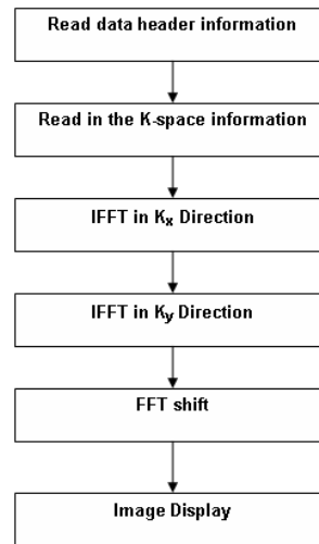
Fig. 5. Flow diagram of IFFT Method of reconstruction
