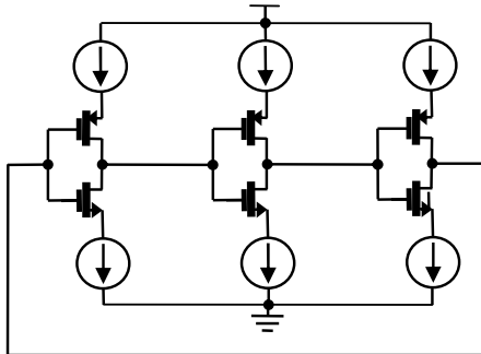
Fig. 5 Current-starved ring oscillator
