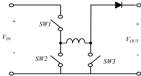
Fig. 2 Modified Buck Boost circuit
