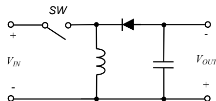
Fig. 1 Buck Boost circuit configuration
