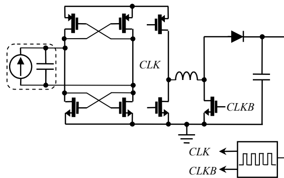
Fig. 4 Modified Buck Boost circuit as linear energy harvester
