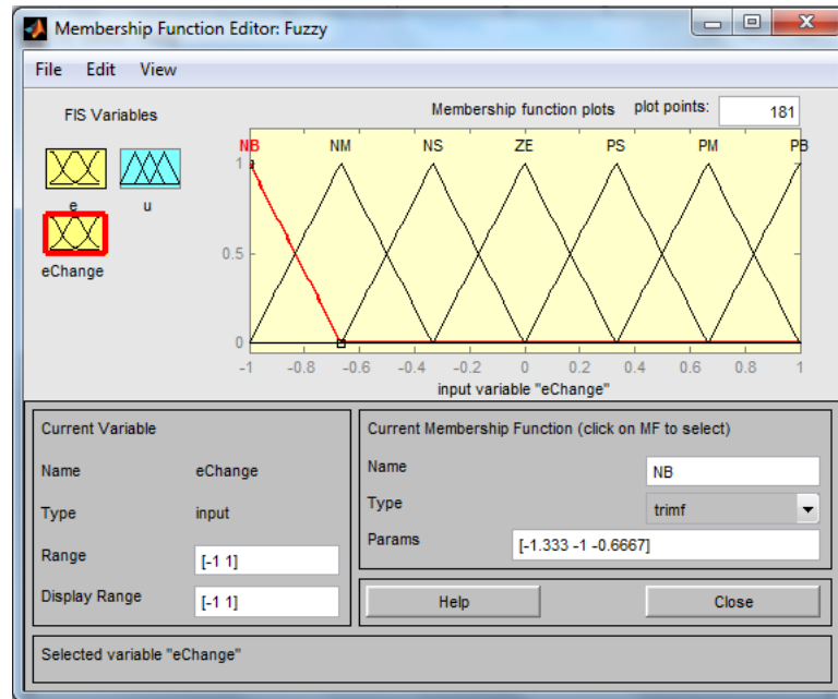
Fig. 10 Membership function for error change (input 2)
