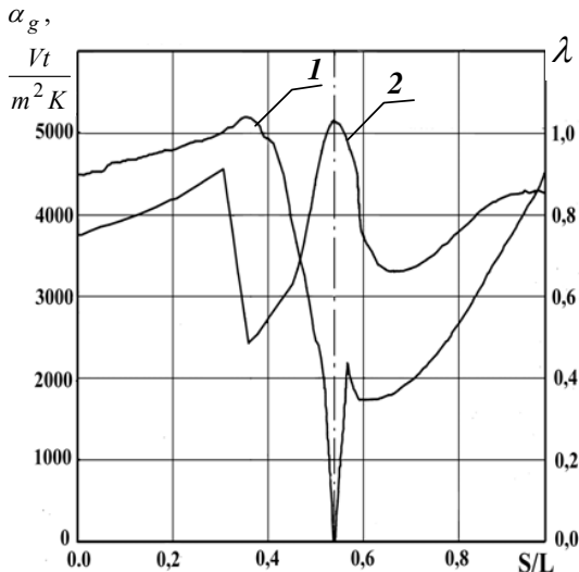
Fig. 4 Distribution of the relative speeds \lambda (1) and of gas convective heat exchange coefficients \alpha_T (2) along the periphery of the profile contour
