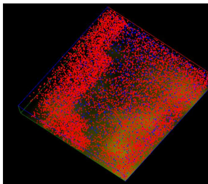
Fig. 23. A sample view of the distribution of chaperones (blue points) and nascent proteins (red points), right-folded proteins (yellow points), misfolded proteins of type 1 (green points) and misfolded proteins of type 2 (magenta points).
