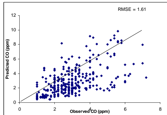
Fig. 2 Observed CO Vs Predicted CO (CALINE4)
